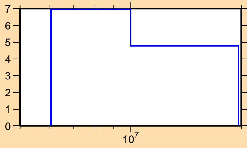
\Delta\sigma/\sigma vs. E for ^{123}\text{Ba}(n,\text{el.})
