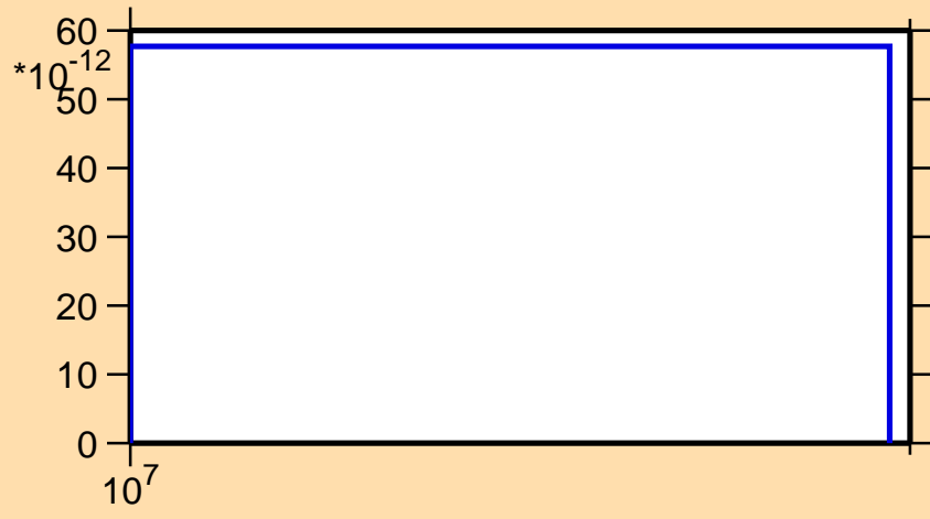
\sigma vs. E for ^{123}\text{Ba}(\text{mt117})
