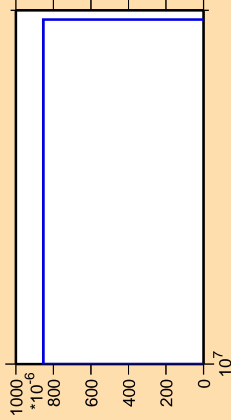
\Delta\sigma/\sigma vs. E for ^{123}\text{Ba}(n,nt)
