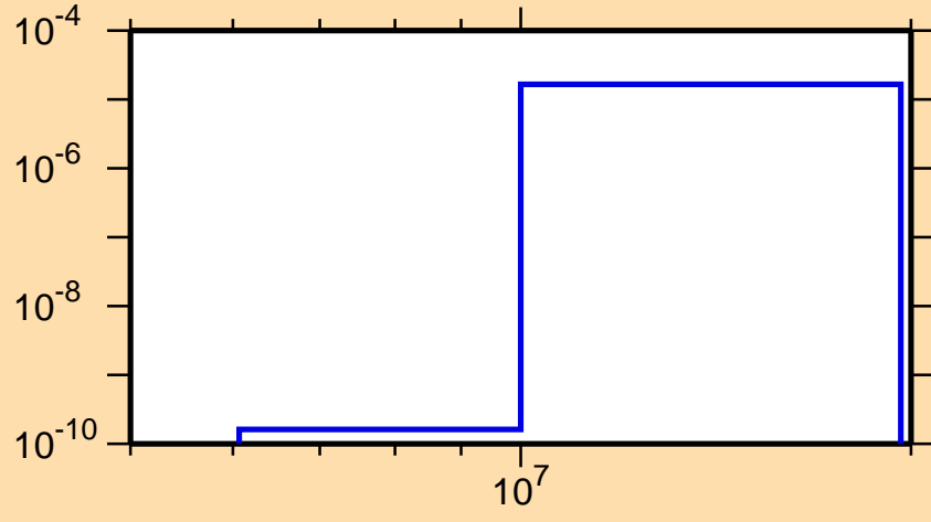
\sigma vs. E for ^{123}\text{Ba}(n,\text{He3})
