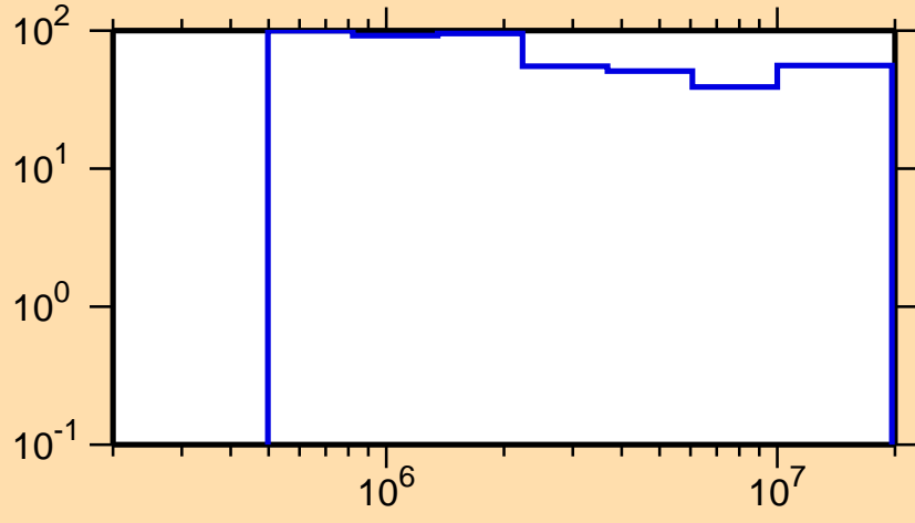
\Delta\sigma/\sigma vs. E for ^{123}\text{Ba}(n,n\text{cont.})
