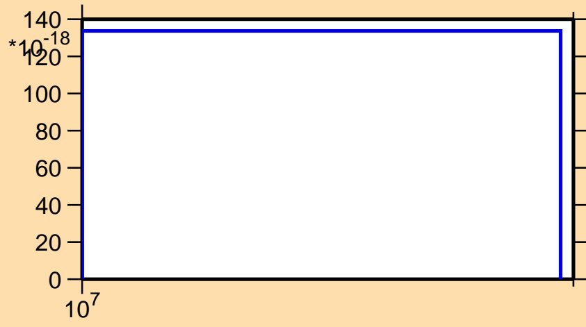
\sigma vs. E for ^{123}\text{Ba}(n,nt)
