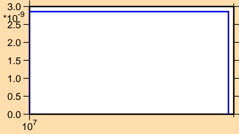
\sigma vs. E for ^{123}\text{Ba} (mt 45)
