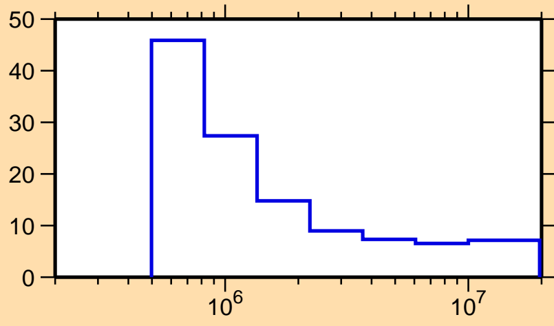
\Delta\sigma/\sigma vs. E for ^{123}\text{Ba}(n,\text{nonel.})
