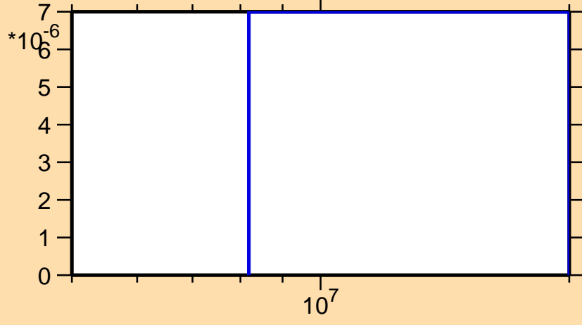
\sigma vs. E for ^{123}\text{Ba}(n,\text{pd})
