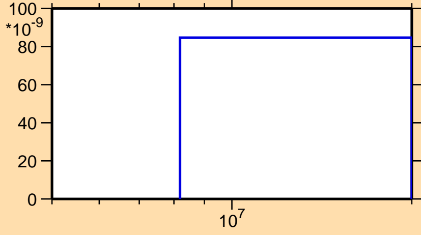
\sigma vs. E for ^{123}\text{Ba}(n,\text{nd})
