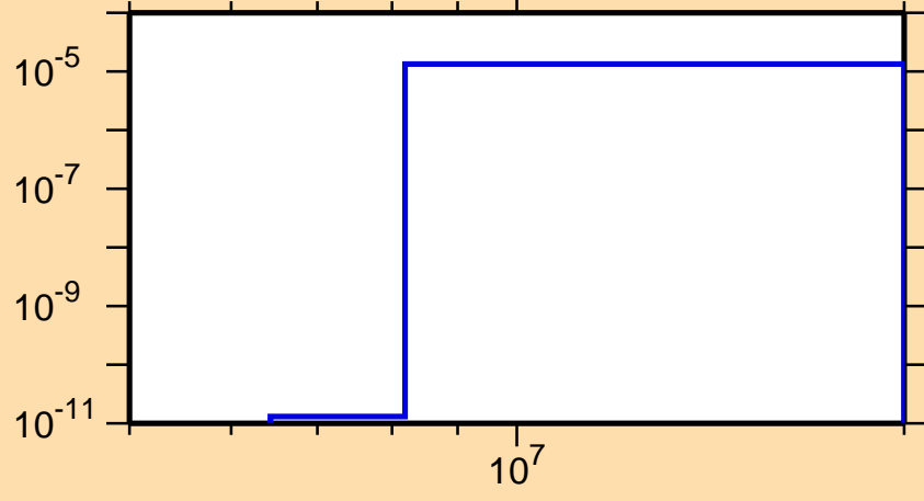
\sigma vs. E for ^{123}\text{Ba}(n,\text{He}3)
