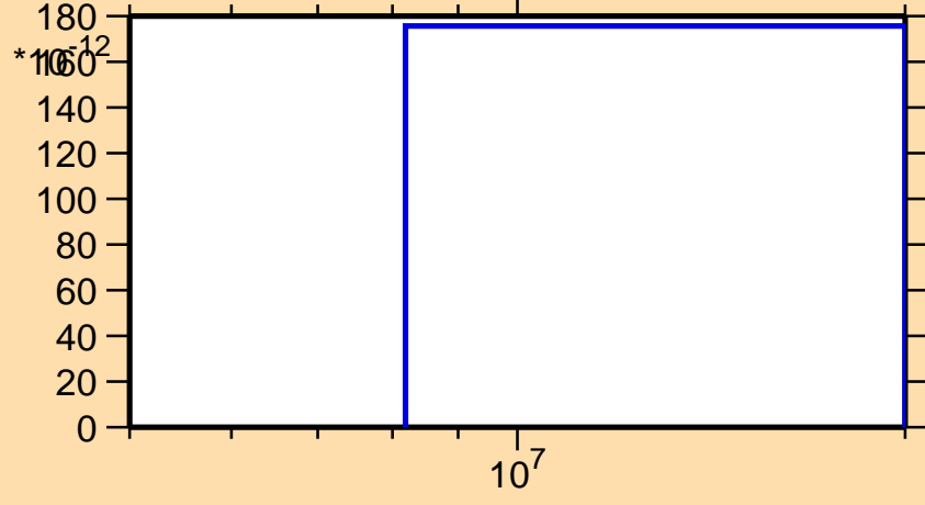
\sigma vs. E for ^{123}\text{Ba} (mt 34)
