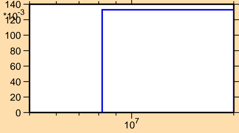
\sigma vs. E for ^{123}\text{Ba}(n,2n)
