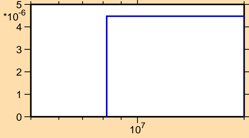
\sigma vs. E for ^{123}\text{Ba}(n,2np)
