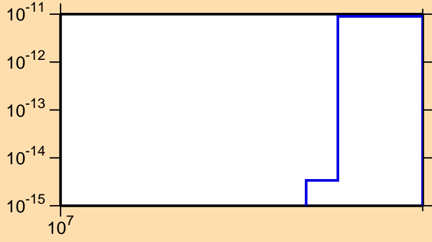
\sigma vs. E for ^{124}\text{Ba} (mt 34)
