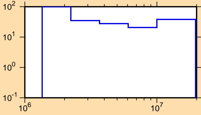
\Delta\sigma/\sigma vs. E for ^{124}\text{Ba}(n,n\text{cont.})
