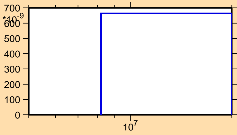
\sigma vs. E for ^{124}\text{Ba}(n,\text{pd})
