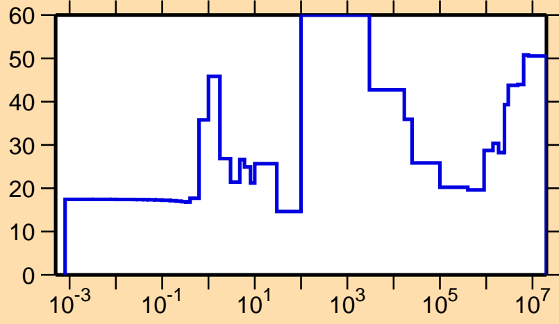
\Delta\sigma/\sigma vs. E for ^{124}\text{Ba}(n,\gamma)
