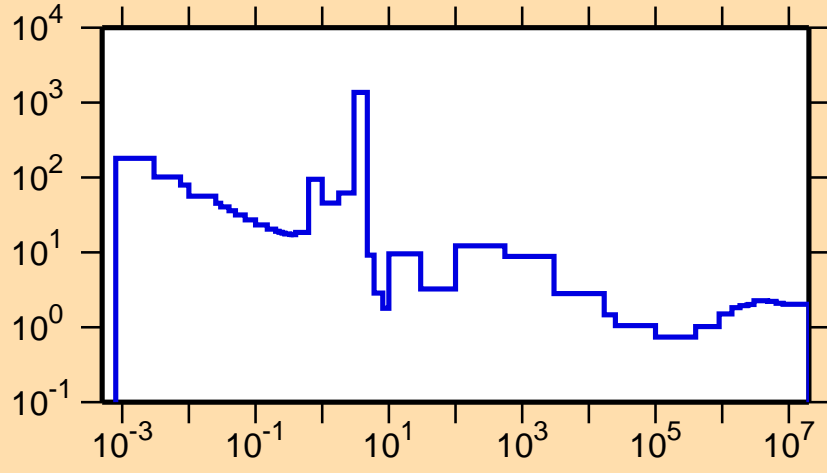
\sigma vs. E for ^{124}\text{Ba}(n,\text{nonel.})
