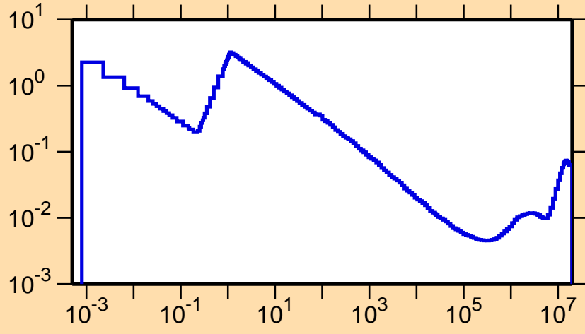
\sigma vs. E for ^{125}\text{Ba}(n,\alpha)
