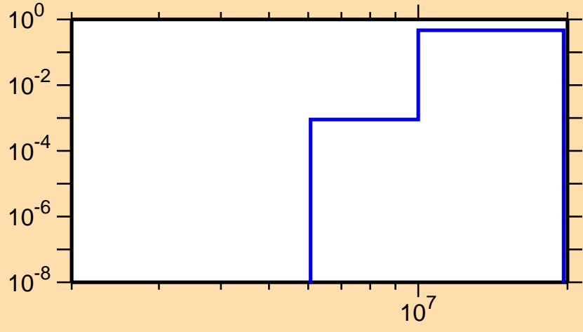
\sigma vs. E for ^{125}\text{Ba}(n,np)
