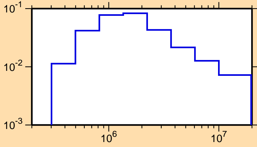
\sigma vs. E for ^{125}\text{Ba}(n,n_3)
