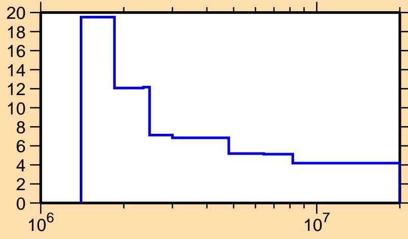
\Delta\sigma/\sigma vs. E for ^{125}\text{Ba}(n,n\text{onel.})
