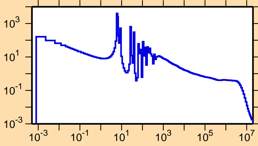
\sigma vs. E for ^{126}\text{Ba}(n,\gamma)
