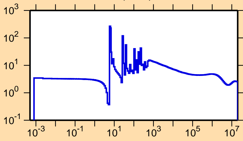
\sigma vs. E for ^{126}\text{Ba}(n,\text{el.})
