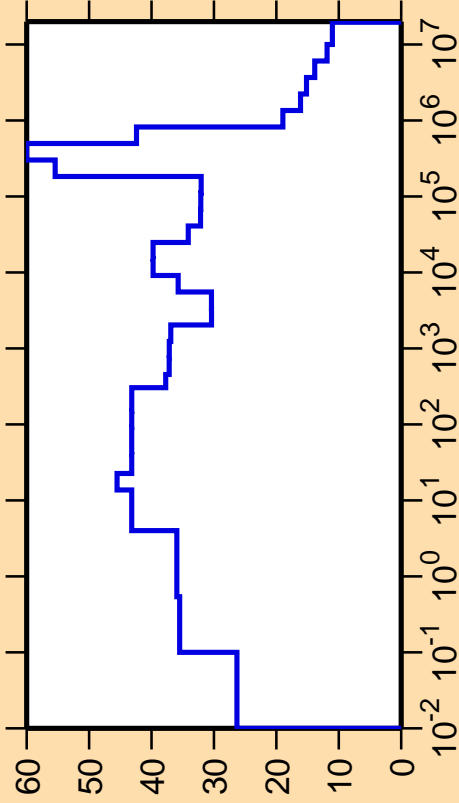
\Delta\sigma/\sigma vs. E for ^{126}\text{Ba}(n,\text{nonel.})
