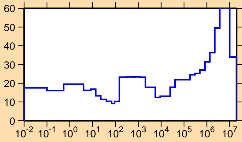
\Delta\sigma/\sigma vs. E for ^{127}\text{Ba}(n,\gamma)
