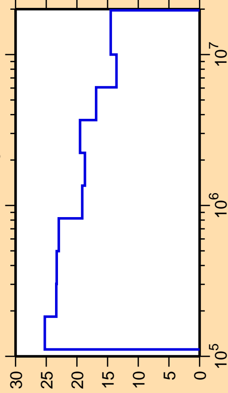
\Delta\sigma/\sigma vs. E for ^{127}\text{Ba}(n,n_3)
