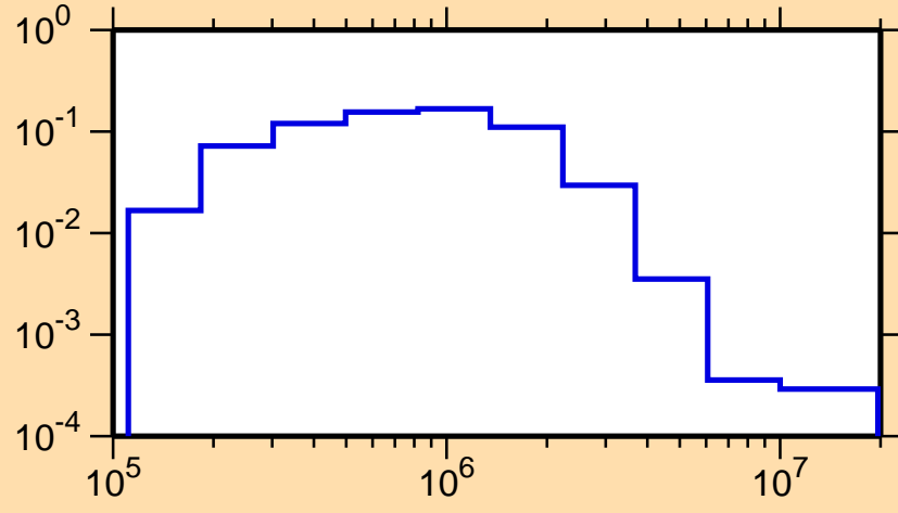
\sigma vs. E for ^{127}\text{Ba}(n,n_3)
