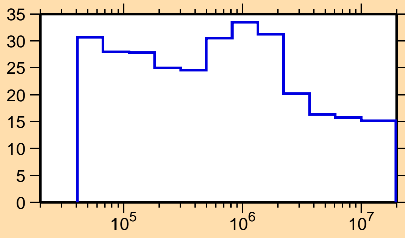
\Delta\sigma/\sigma vs. E for ^{127}\text{Ba}(n,n_1)
