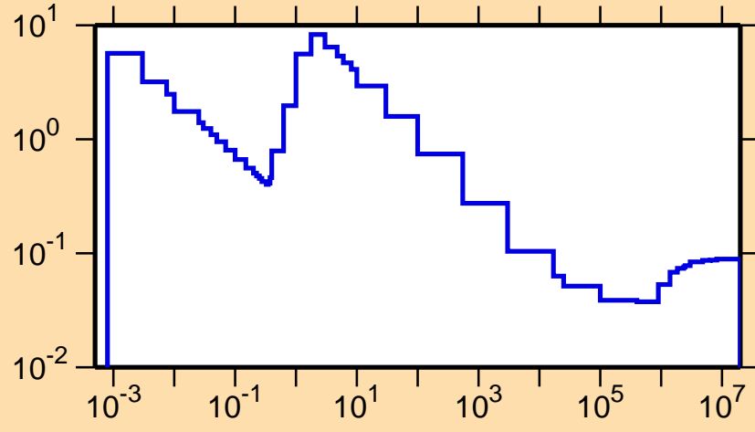
\sigma vs. E for ^{127}\text{Ba}(n,p)
