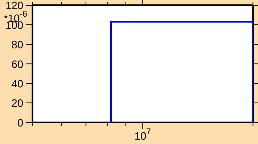
\sigma vs. E for ^{127}\text{Ba}(n,t)
