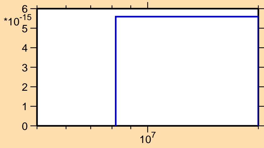
\sigma vs. E for ^{128}\text{Ba}(n,\text{pt})
