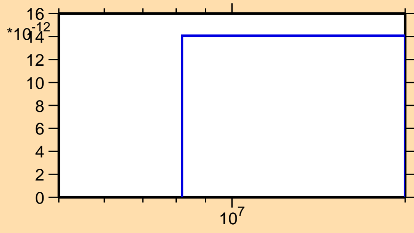
\sigma vs. E for ^{129}\text{Ba}(n,pt)
