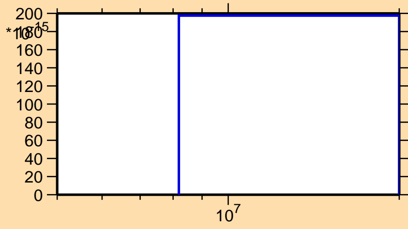
\sigma vs. E for ^{129}\text{Ba}(\text{mt } 34)
