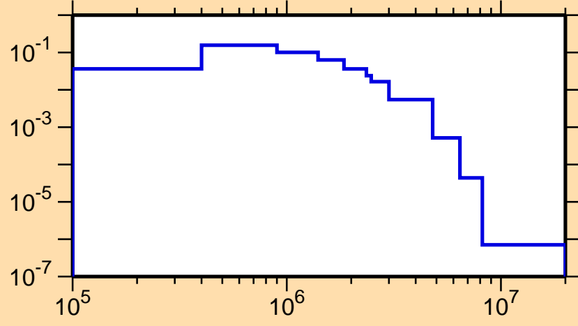
\sigma vs. E for ^{129}\text{Ba}(n,n_4)
