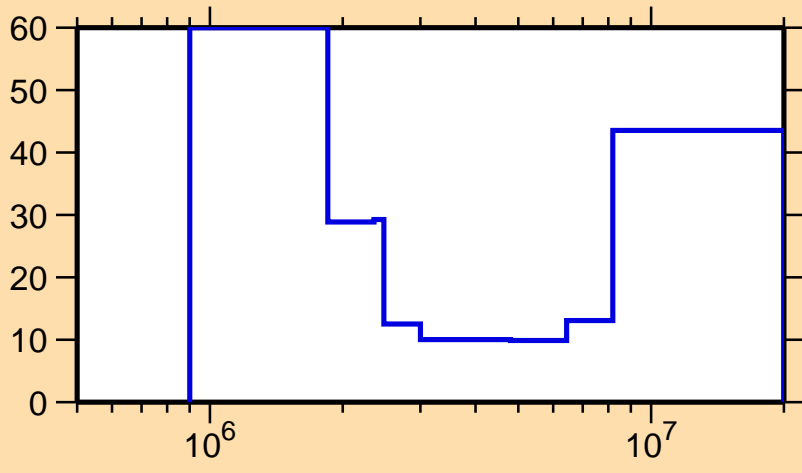
\Delta\sigma/\sigma vs. E for ^{129}\text{Ba}(n,n\text{cont.})
