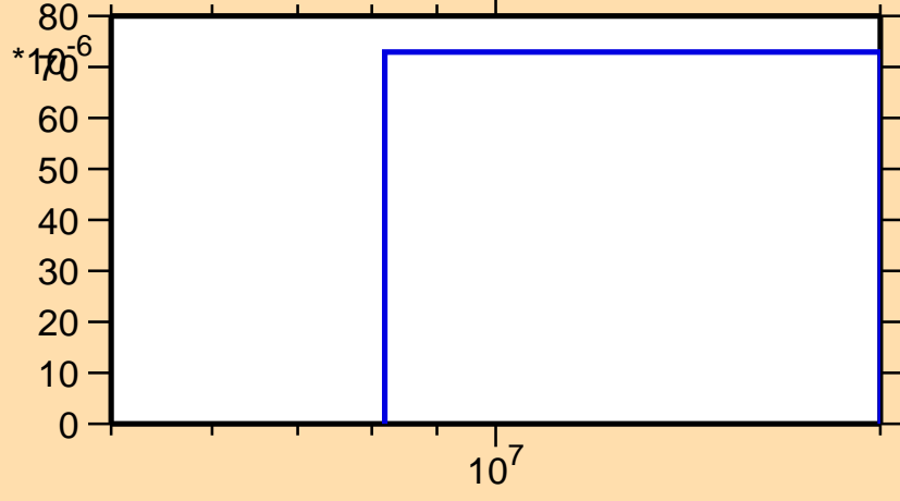
\sigma vs. E for ^{129}\text{Ba}(n,t)
