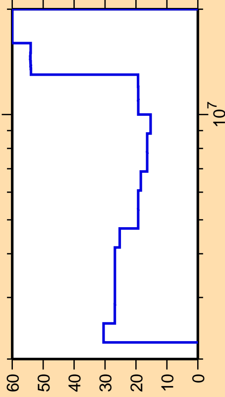
\Delta\sigma/\sigma vs. E for ^{130}\text{Ba}(n,n\text{cont.})
