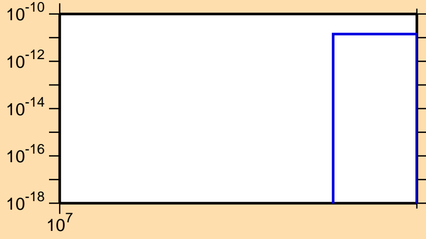
\sigma vs. E for ^{130}\text{Ba}(n,nt)
