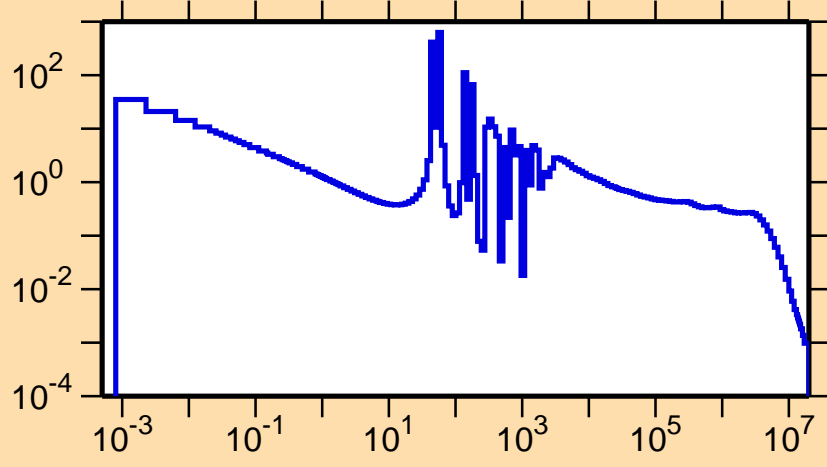
\sigma vs. E for ^{130}\text{Ba}(n,\gamma)
