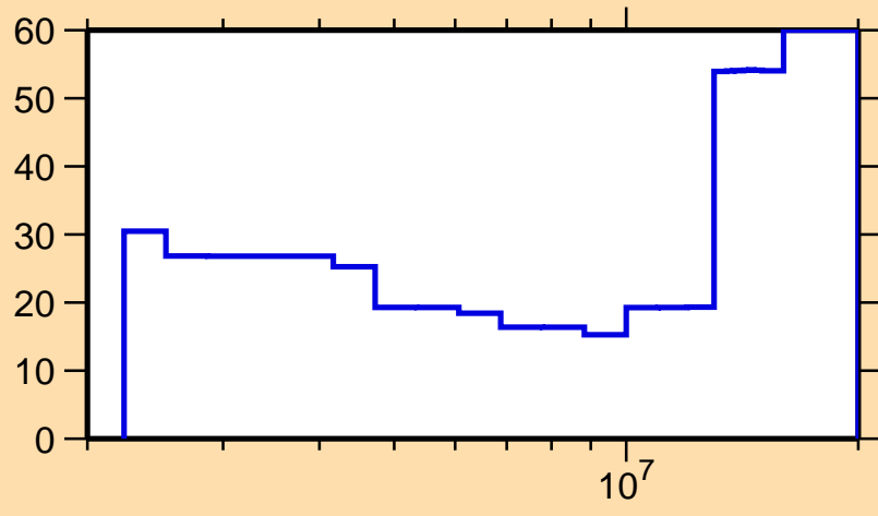
\Delta\sigma/\sigma vs. E for ^{130}\text{Ba}(n,n\text{cont.})
