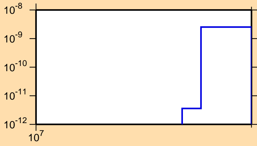
\sigma vs. E for ^{130}\text{Ba}(n,2n\alpha)
