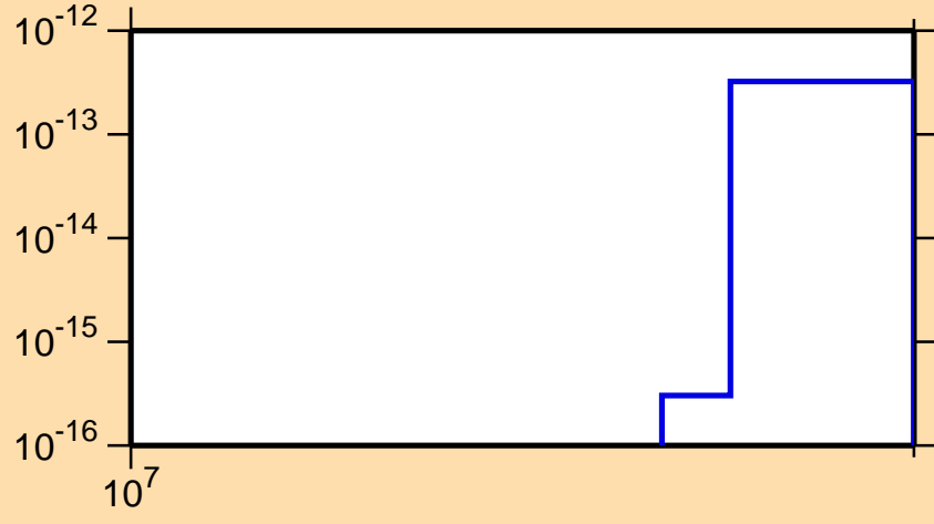
\sigma vs. E for ^{130}\text{Ba} (mt 45)
