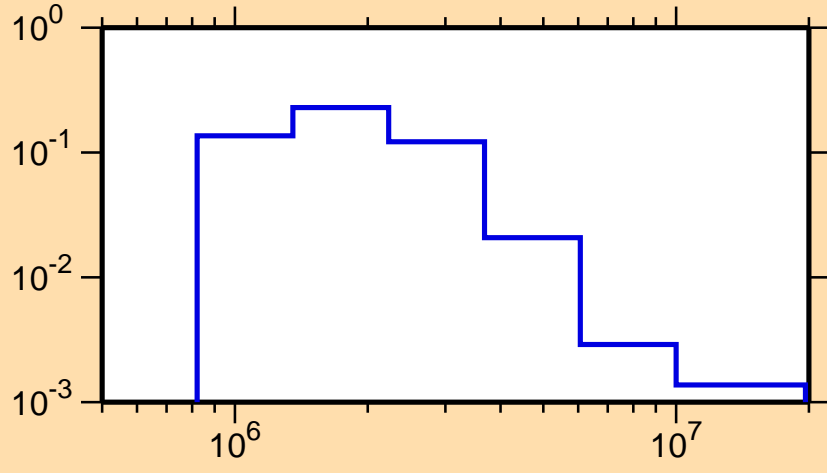
\sigma vs. E for ^{130}\text{Ba}(n,n_4)
