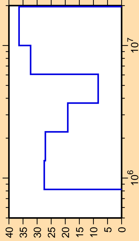
\Delta\sigma/\sigma vs. E for ^{130}\text{Ba}(n,n_4)
