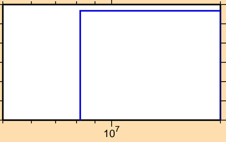
\sigma vs. E for ^{130}\text{Ba}(n,t)
