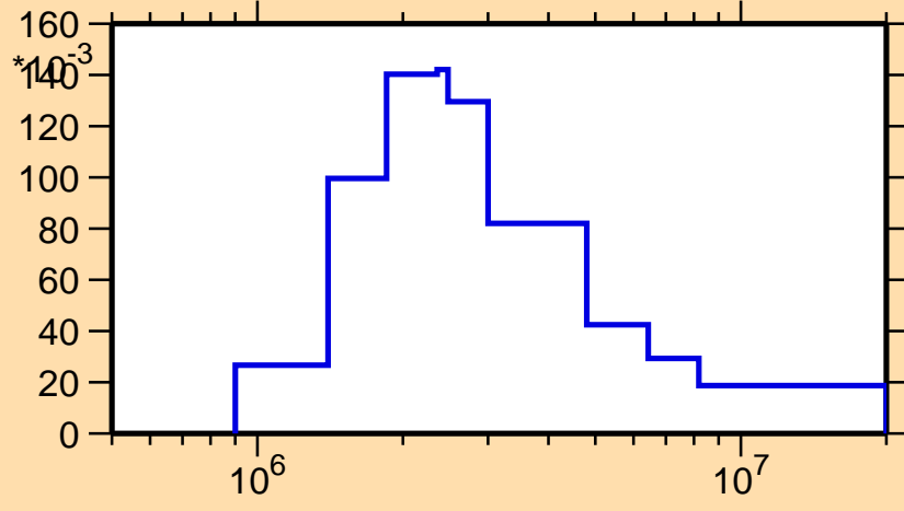
\sigma vs. E for ^{130}\text{Ba}(n,n_3)
