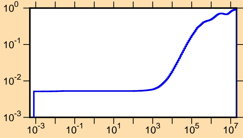
\mu vs. E for ^{131}\text{Ba}(\text{mt251})
