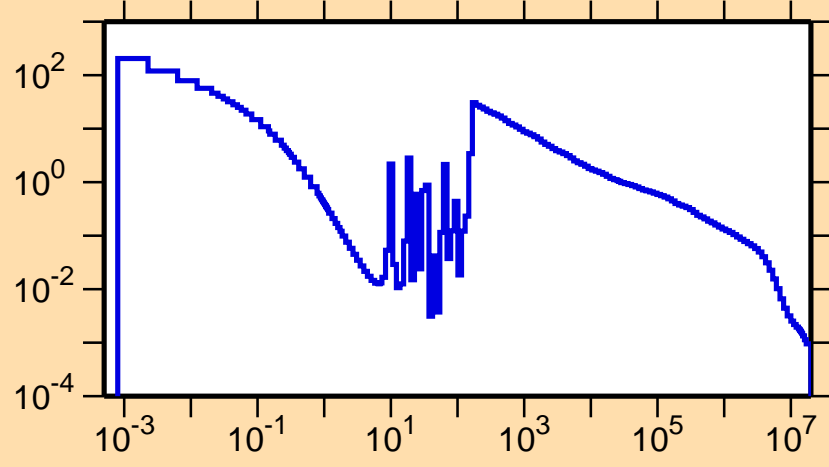
\sigma vs. E for ^{131}\text{Ba}(n,\gamma)
