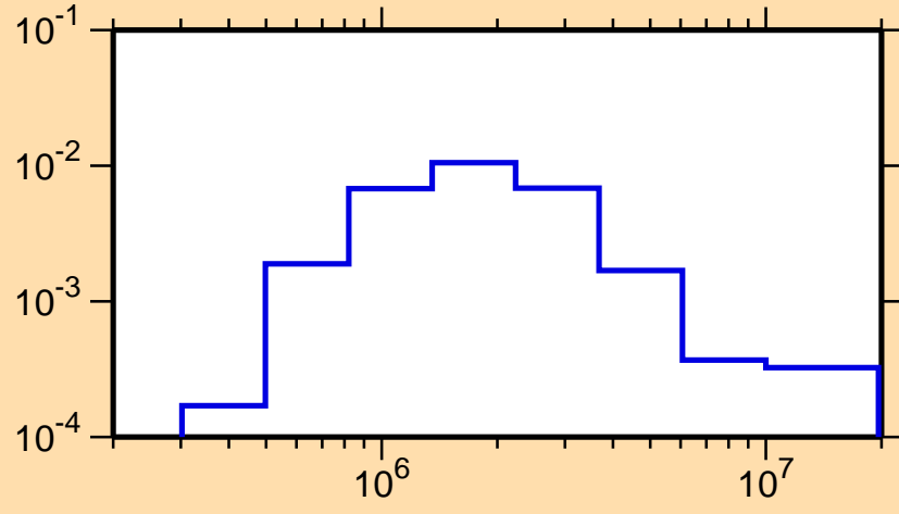
\sigma vs. E for ^{131}\text{Ba}(n,n_4)
