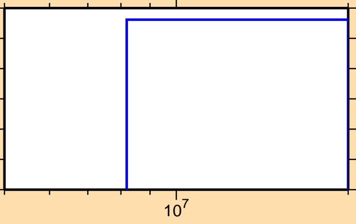
\sigma vs. E for ^{131}\text{Ba}(n,\text{nd})
