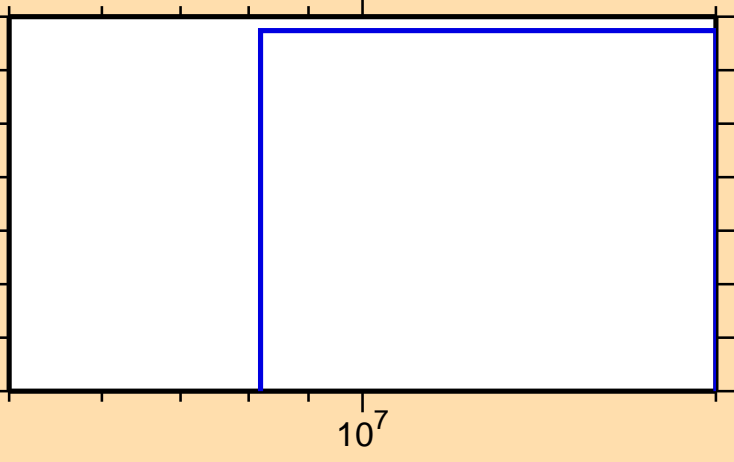
\sigma vs. E for ^{131}\text{Ba}(n,nt)
