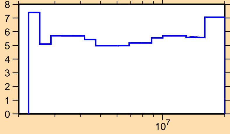
\Delta\sigma/\sigma vs. E for ^{132}\text{Ba}(n,\text{nonel.})
