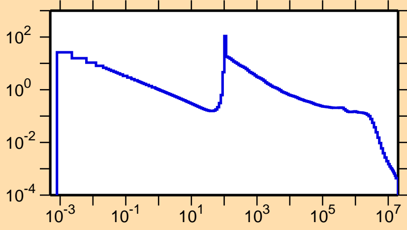
\sigma vs. E for ^{132}\text{Ba}(n,\gamma)
