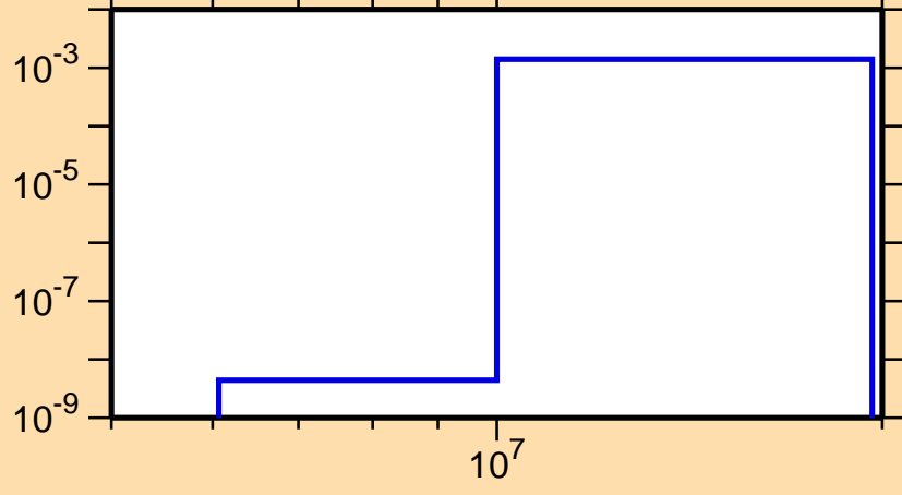
\sigma vs. E for ^{132}\text{Ba}(n,d)
