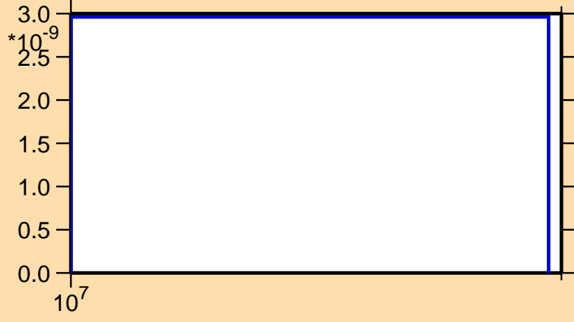
\sigma vs. E for ^{132}\text{Ba}(n,\text{He}3)
