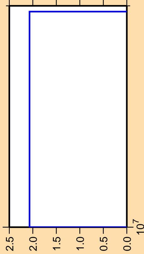
\Delta\sigma/\sigma vs. E for ^{132}\text{Ba}(n,\text{pd})
