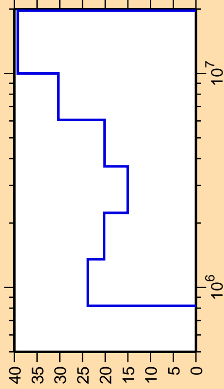
\Delta\sigma/\sigma vs. E for ^{132}\text{Ba}(n,n_2)
