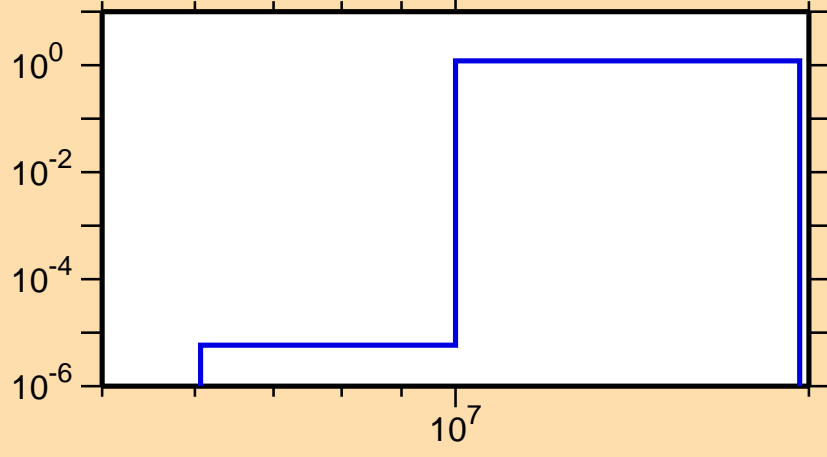
\sigma vs. E for ^{132}\text{Ba}(n,2n)
