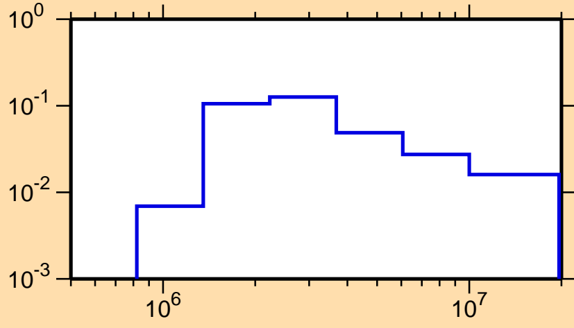
\sigma vs. E for ^{132}\text{Ba}(n,n_3)
