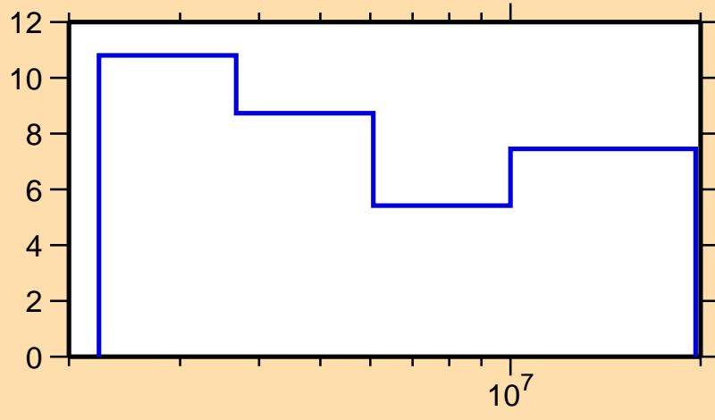
\Delta\sigma/\sigma vs. E for ^{132}\text{Ba}(n,\text{el.})
