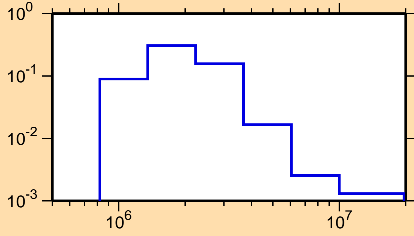
\sigma vs. E for ^{132}\text{Ba}(n,n_2)
