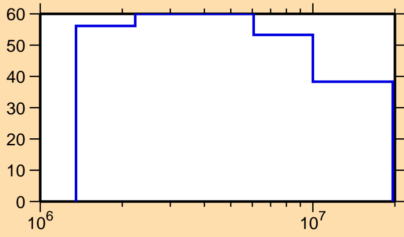
\Delta\sigma/\sigma vs. E for ^{132}\text{Ba}(n,p)
