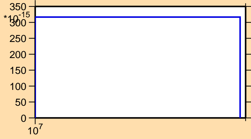
\sigma vs. E for ^{132}\text{Ba}(n,\text{pd})
