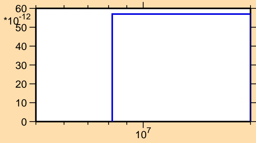
\sigma vs. E for ^{132}\text{Ba}(n,p\alpha)
