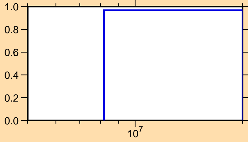
\sigma vs. E for ^{132}\text{Ba}(n,2n)
