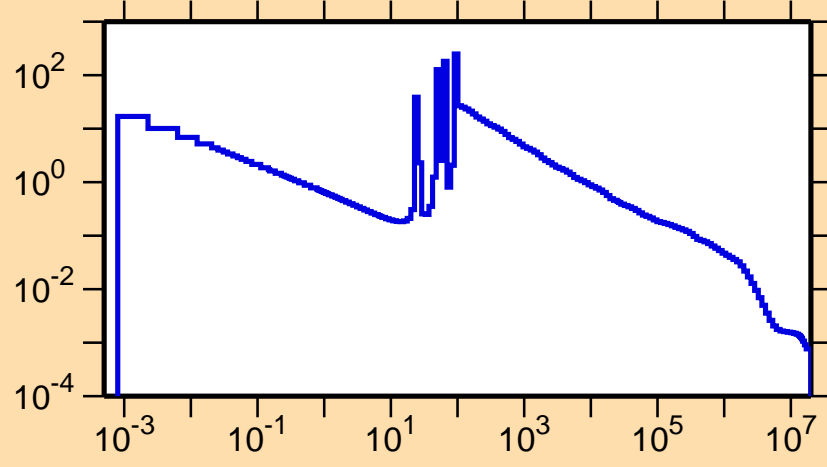
\sigma vs. E for ^{133}\text{Ba}(n,\gamma)
