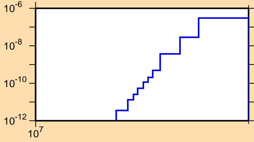
\sigma vs. E for ^{133}\text{Ba}(n,\text{He3})
