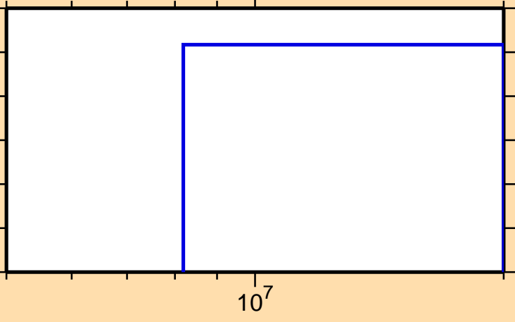
\sigma vs. E for ^{133}\text{Ba}(n,2np)
