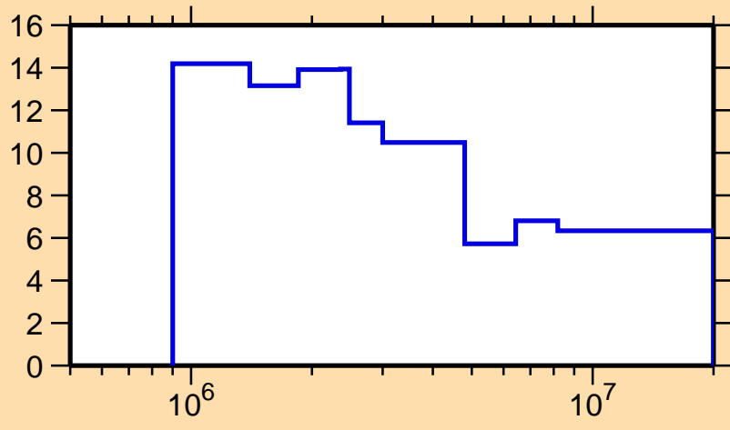
\Delta\sigma/\sigma vs. E for ^{133}\text{Ba}(n,n\text{onel.})
