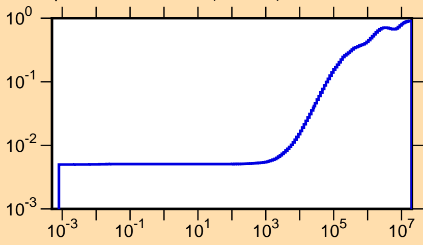
\mu vs. E for ^{135}\text{Ba}(\text{mt251})
