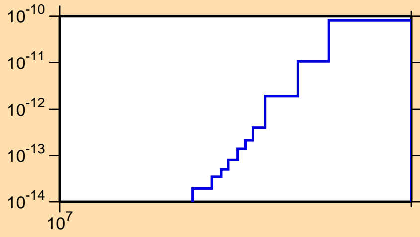
\sigma vs. E for ^{135}\text{Ba}(n,p\alpha)
