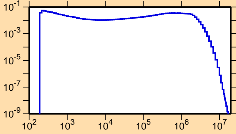
\sigma vs. E for ^{135}\text{Ba}(n,n_1)
