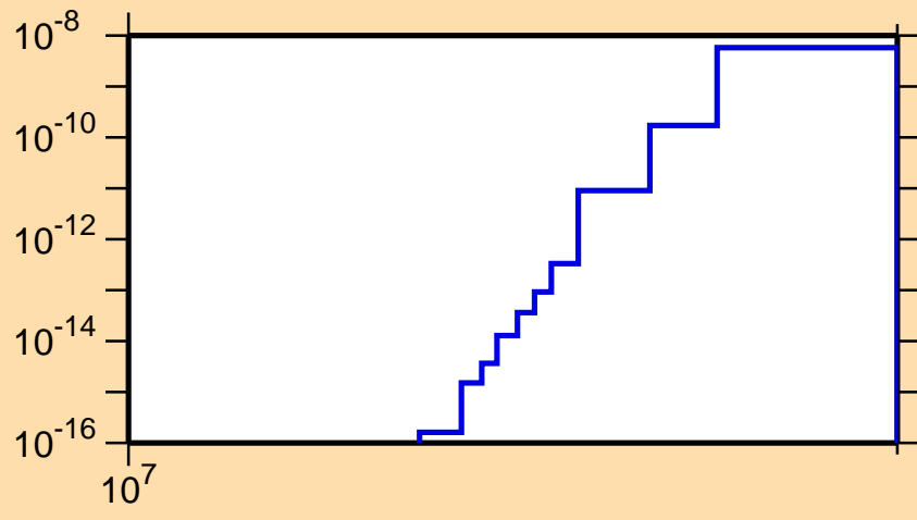
\sigma vs. E for ^{135}\text{Ba}(n,\text{He3})
