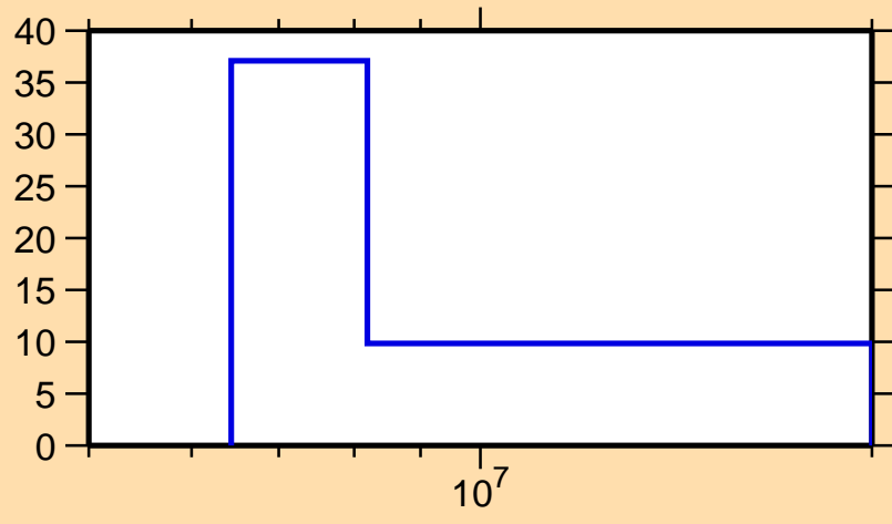
\Delta\sigma/\sigma vs. E for ^{135}\text{Ba}(n,2n)
