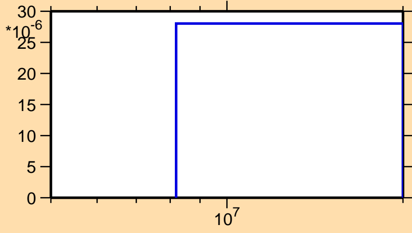
\sigma vs. E for ^{135}\text{Ba}(n,t)
