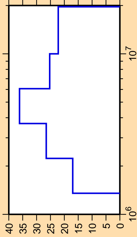
\Delta\sigma/\sigma vs. E for ^{136}\text{Ba}(n,n_2)
