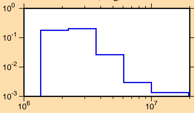
\sigma vs. E for ^{136}\text{Ba}(n,n_2)
