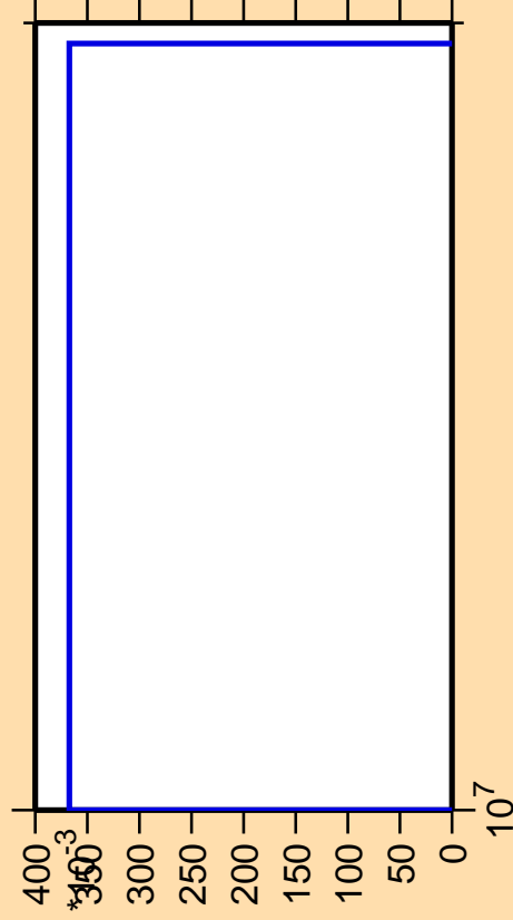
\Delta\sigma/\sigma vs. E for ^{136}\text{Ba}(n,2n\alpha)
