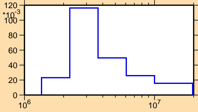
\sigma vs. E for ^{136}\text{Ba}(n,n_4)
