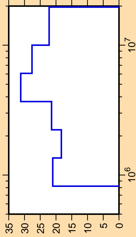
\Delta\sigma/\sigma vs. E for ^{136}\text{Ba}(n,n_1)
