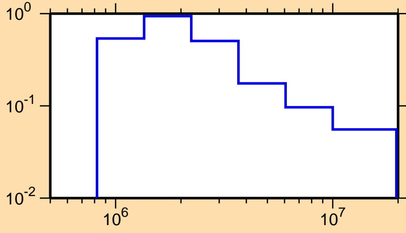
\sigma vs. E for ^{136}\text{Ba}(n,n_1)
