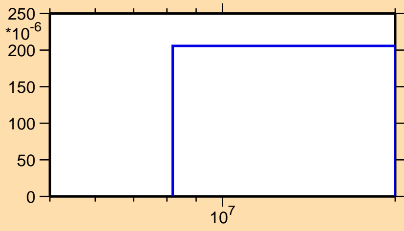
\sigma vs. E for ^{136}\text{Ba}(n,3n)
