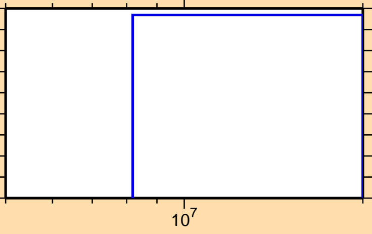
\sigma vs. E for ^{136}\text{Ba}(n,\text{nd})
