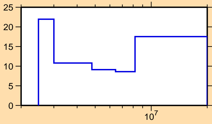
\Delta\sigma/\sigma vs. E for ^{136}\text{Ba}(n,n\text{cont.})
