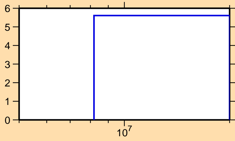
\Delta\sigma/\sigma vs. E for ^{136}\text{Ba}(n,\text{nonel.})
