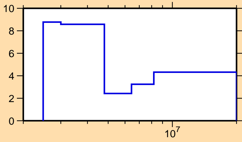
\Delta\sigma/\sigma vs. E for ^{136}\text{Ba}(n,\text{el.})
