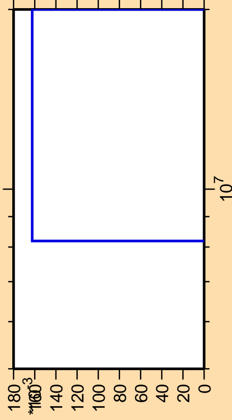
\Delta\sigma/\sigma vs. E for ^{136}\text{Ba}(n,2np)
