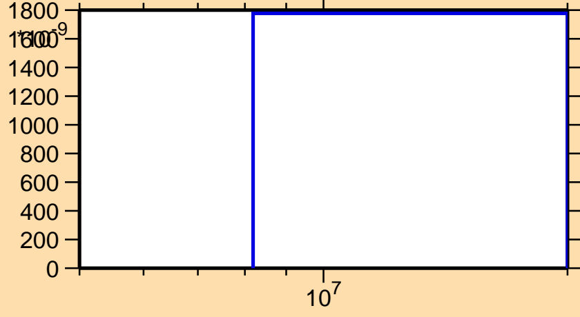
\sigma vs. E for ^{136}\text{Ba}(n,t)
