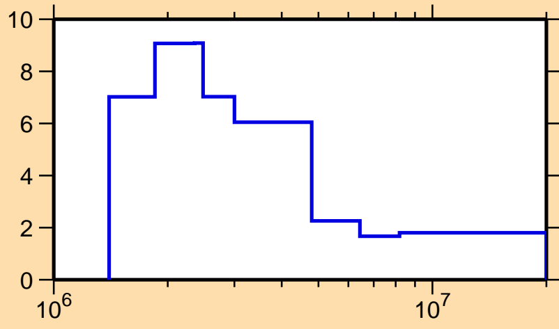
\Delta\sigma/\sigma vs. E for ^{136}\text{Ba}(n,\text{tot.})
