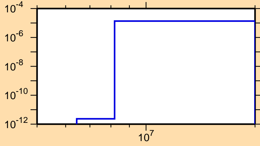
\sigma vs. E for ^{136}\text{Ba}(n,n\alpha)
