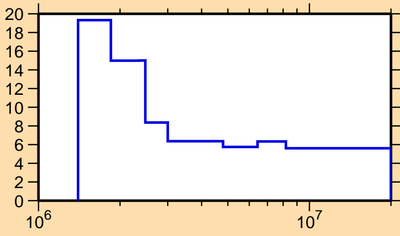
\Delta\sigma/\sigma vs. E for ^{136}\text{Ba}(n,\text{nonel.})
