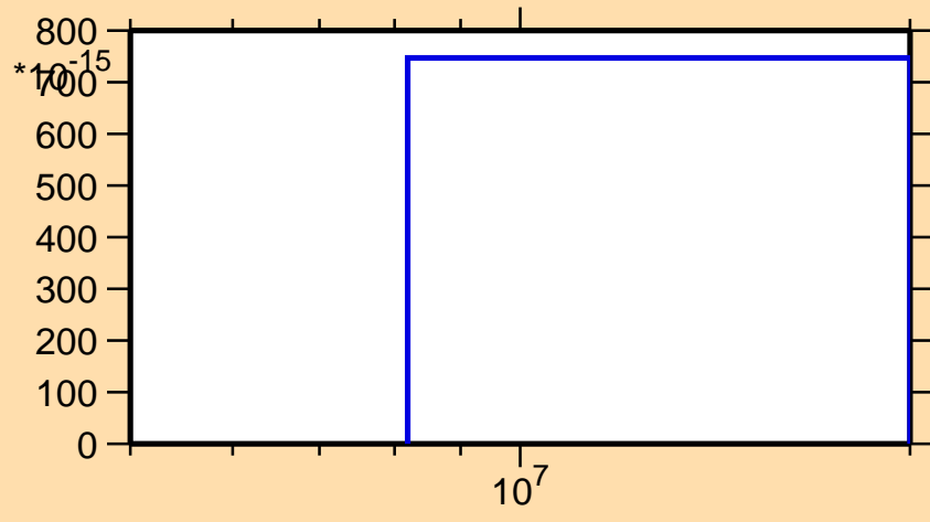
\sigma vs. E for ^{136}\text{Ba}(n,2n\alpha)
