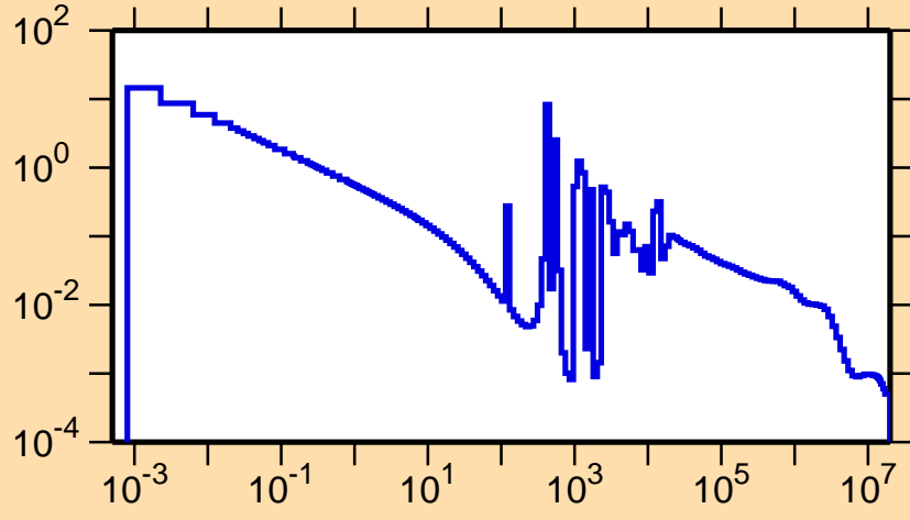
\sigma vs. E for ^{137}\text{Ba}(n,\gamma)
