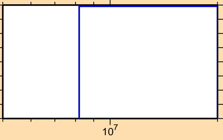
\sigma vs. E for ^{137}\text{Ba}(n,t)
