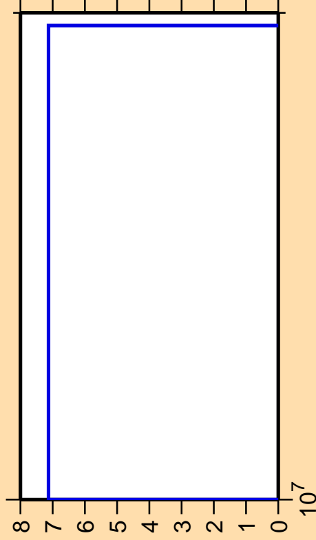
\Delta\sigma/\sigma vs. E for ^{137}\text{Ba}(n,nt)
