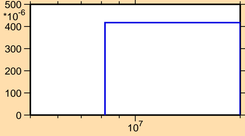
\sigma vs. E for ^{137}\text{Ba}(n,d)
