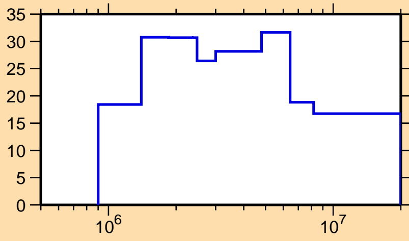
\Delta\sigma/\sigma vs. E for ^{137}\text{Ba}(n,p)
