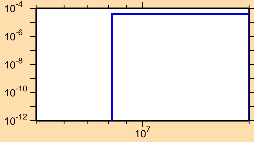
\sigma vs. E for ^{138}\text{Ba}(n,n\alpha)
