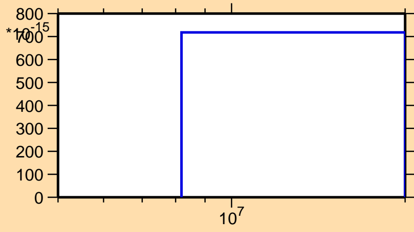
\sigma vs. E for ^{138}\text{Ba}(n,nt)
