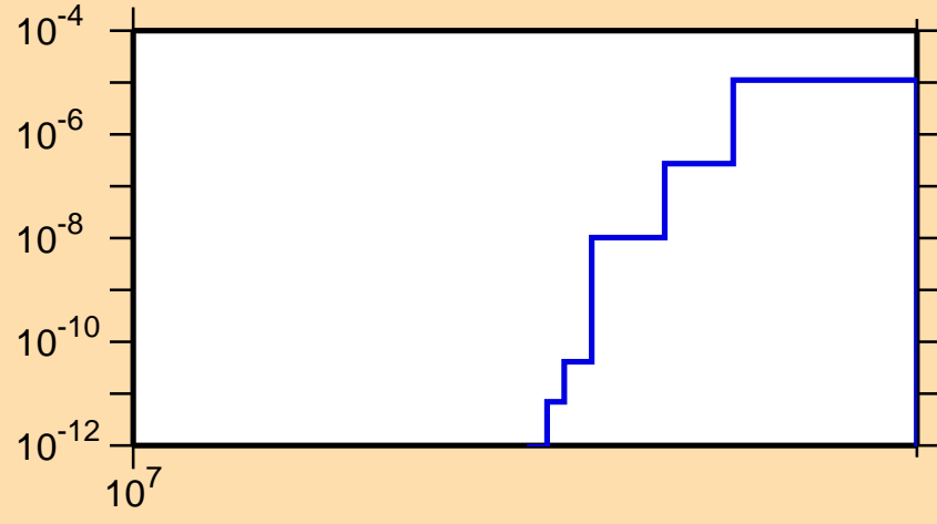
\sigma vs. E for ^{140}\text{Ba}(n,nt)
