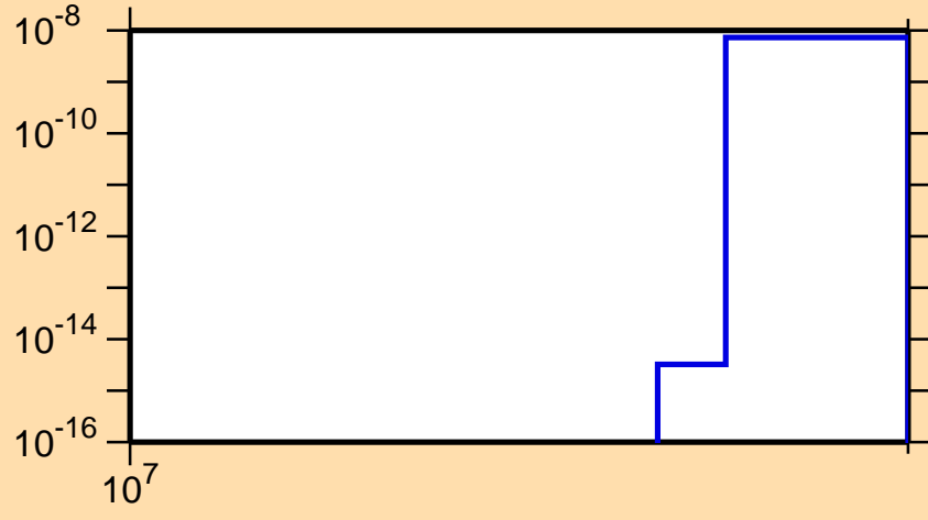
\sigma vs. E for ^{140}\text{Ba}(n,2np)
