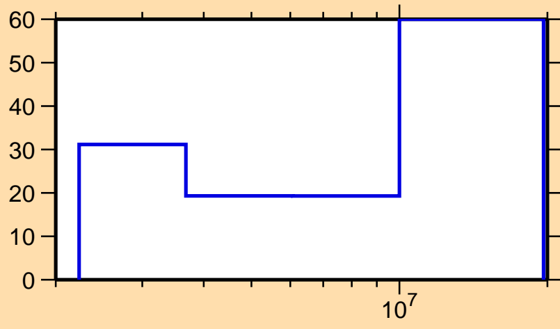
\Delta\sigma/\sigma vs. E for ^{140}\text{Ba}(n,n\text{cont.})
