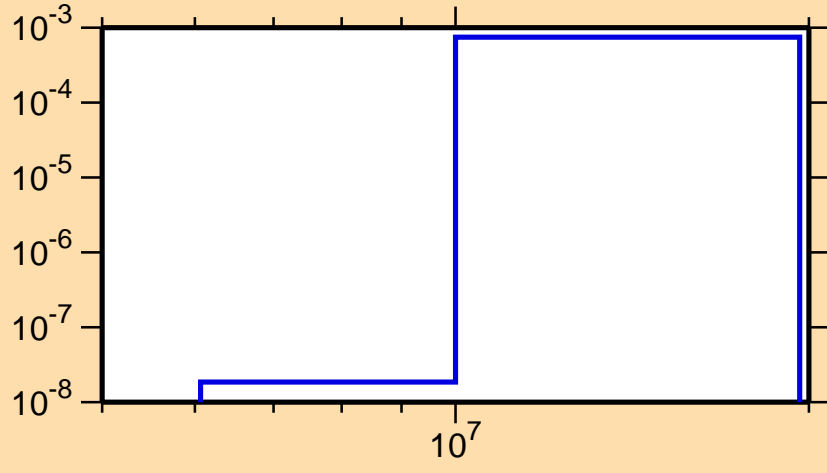
\sigma vs. E for ^{140}\text{Ba}(n,p)
