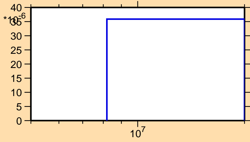
\sigma vs. E for ^{140}\text{Ba}(n,t)
