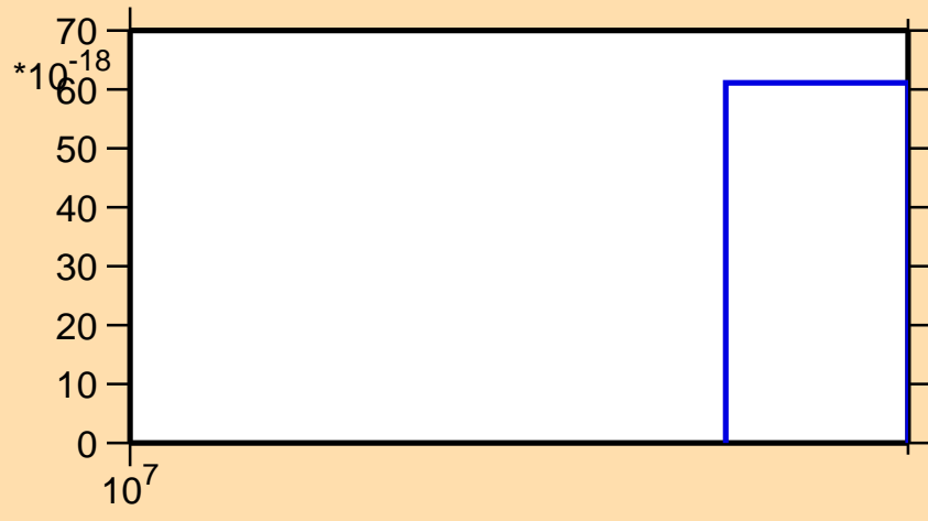
\sigma vs. E for ^{143}\text{Ba} (mt 11)
