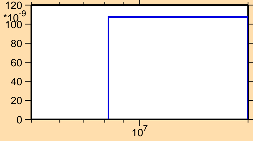
\sigma vs. E for ^{143}\text{Ba}(n,2n\alpha)
