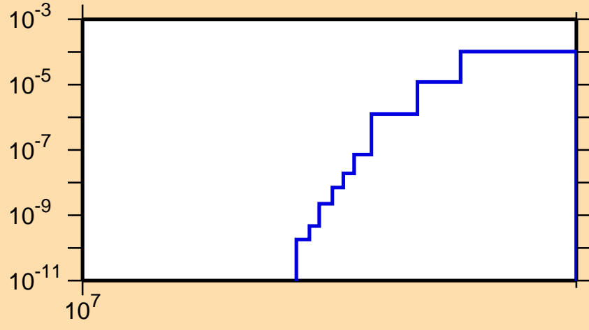
\sigma vs. E for ^{144}\text{Ba}(n,np)
