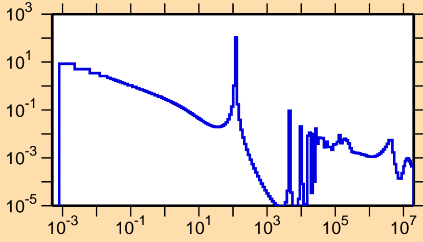
\sigma vs. E for ^{144}\text{Ba}(n,\gamma)
