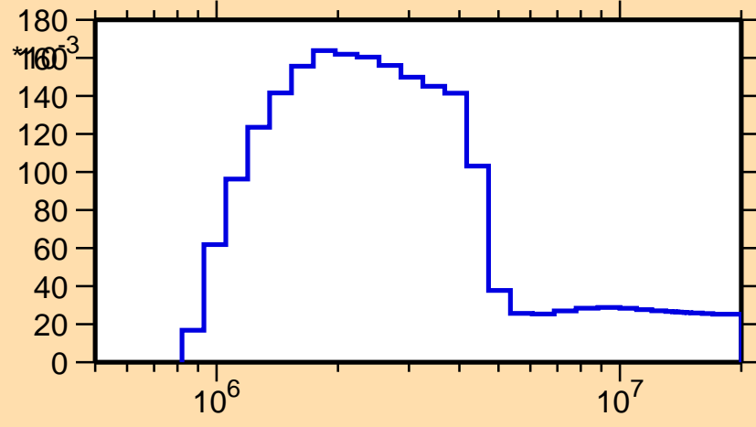
\sigma vs. E for ^{144}\text{Ba}(n,n_4)
