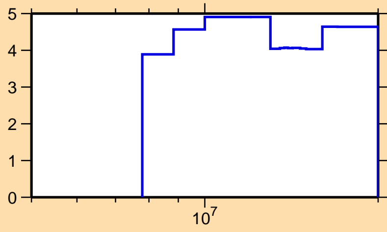
\Delta\sigma/\sigma vs. E for ^{144}\text{Ba}(n,\text{nonel.})
