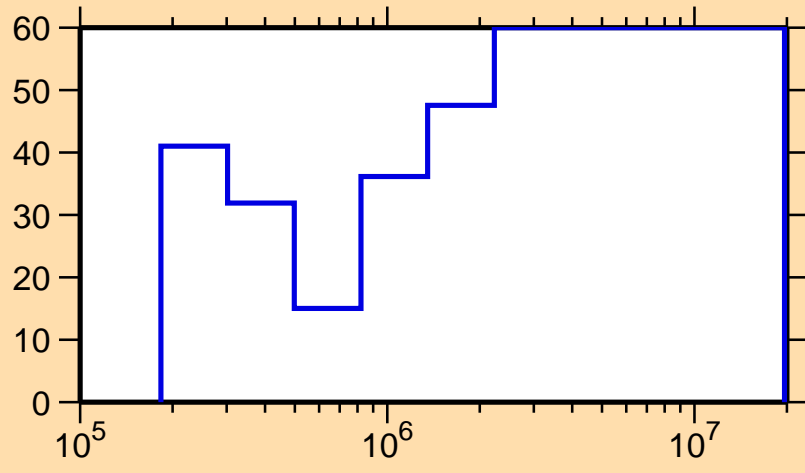
\Delta\sigma/\sigma vs. E for ^{144}\text{Ba}(n,n_1)
