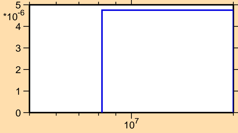
\sigma vs. E for ^{144}\text{Ba}(n,d)
