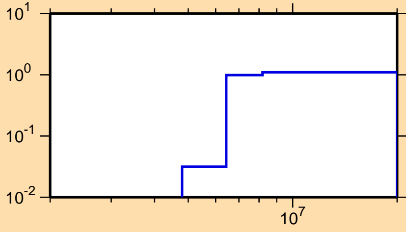
\sigma vs. E for ^{144}\text{Ba}(n,2n)
