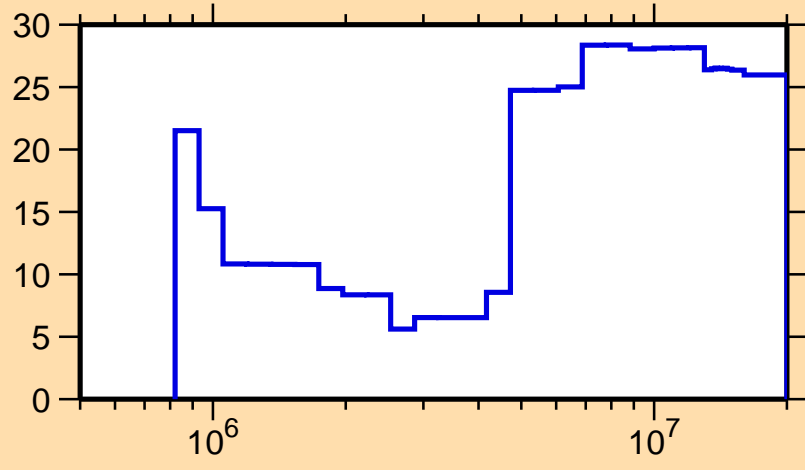
\Delta\sigma/\sigma vs. E for ^{145}\text{Ba}(n,\text{inel.})
