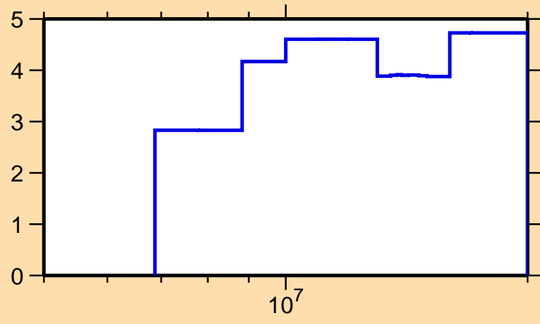
\Delta\sigma/\sigma vs. E for ^{145}\text{Ba}(n,\text{nonel.})
