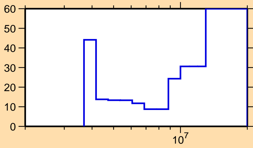
\Delta\sigma/\sigma vs. E for ^{145}\text{Ba}(n,2n)
