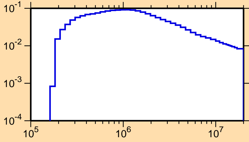
\sigma vs. E for ^{145}\text{Ba}(n,n_2)
