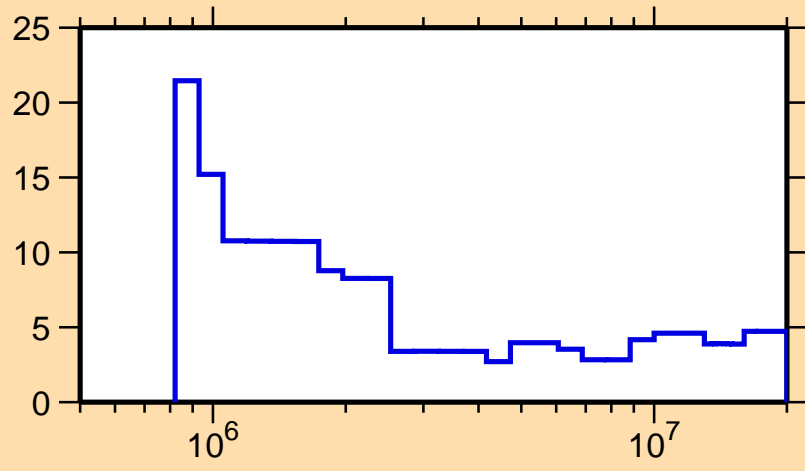
\Delta\sigma/\sigma vs. E for ^{145}\text{Ba}(n,\text{nonel.})
