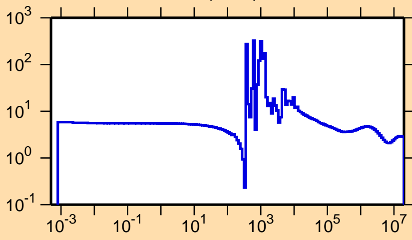
\sigma vs. E for ^{145}\text{Ba}(n,\text{el.})
