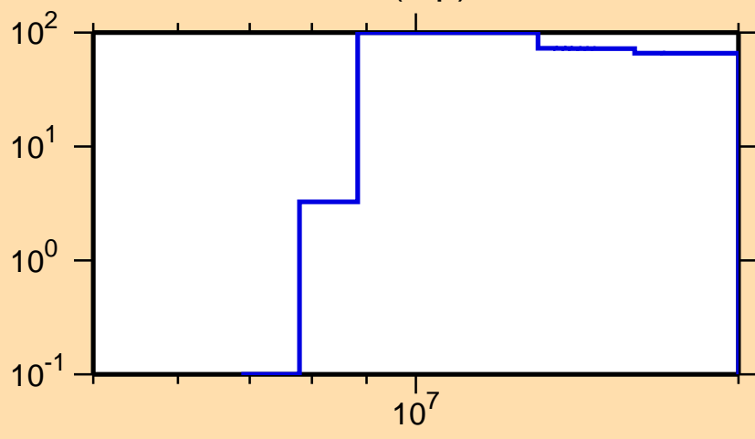
\Delta\sigma/\sigma vs. E for ^{145}\text{Ba}(n,p)
