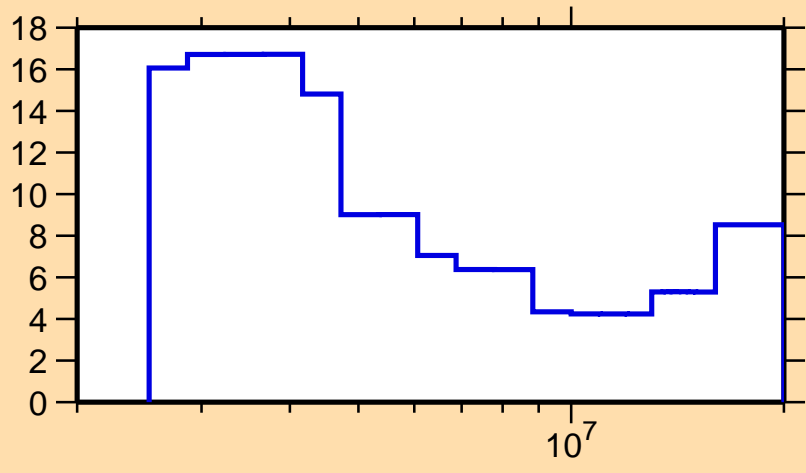
\Delta\sigma/\sigma vs. E for ^{145}\text{Ba}(n,\text{el.})
