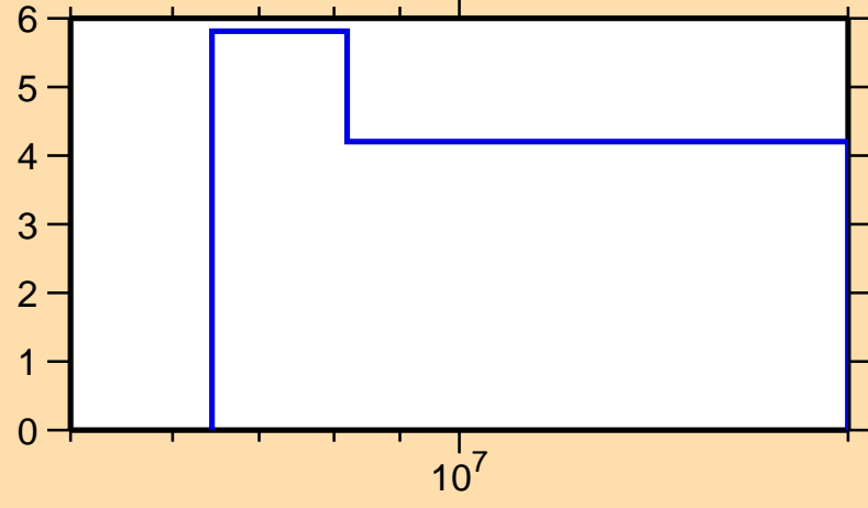
\Delta\sigma/\sigma vs. E for ^{145}\text{Ba}(n,\text{el.})
