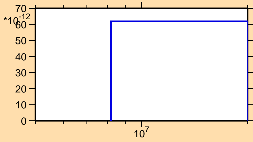
\sigma vs. E for ^{145}\text{Ba}(n,2np)
