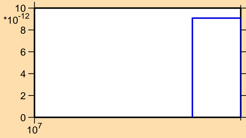
\sigma vs. E for ^{146}\text{Ba}(n,2np)
