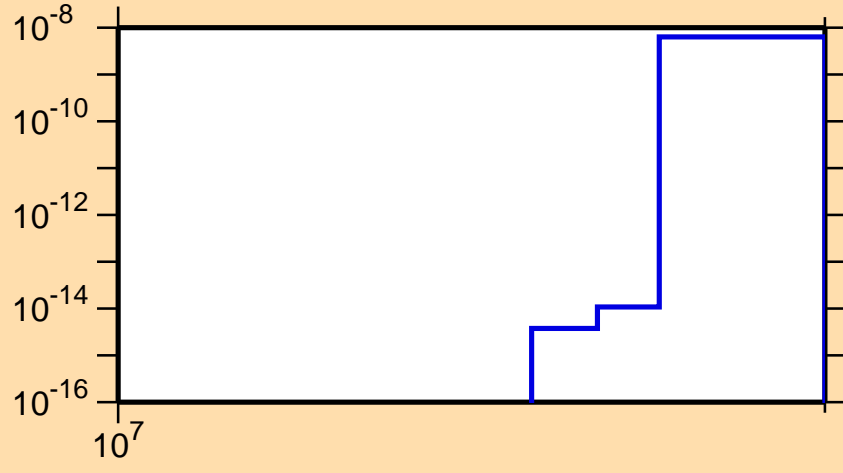
\sigma vs. E for ^{146}\text{Ba}(n,\text{nd})
