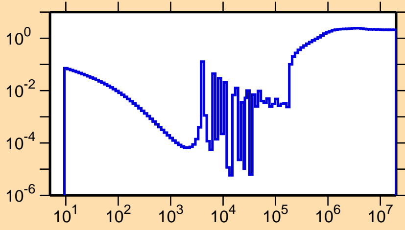
\sigma vs. E for ^{146}\text{Ba}(n,\text{nonel.})
