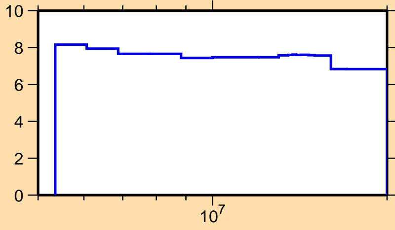
\Delta\sigma/\sigma vs. E for ^{146}\text{Ba}(n,\text{nonel.})
