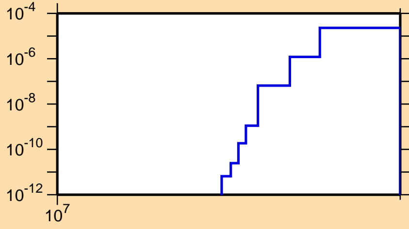
\sigma vs. E for ^{146}\text{Ba}(n,np)
