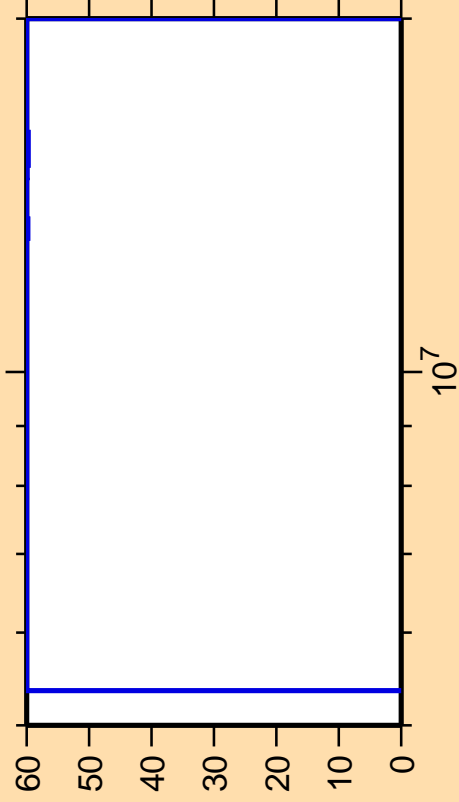
\Delta\sigma/\sigma vs. E for ^{146}\text{Ba}(n,n_1)
